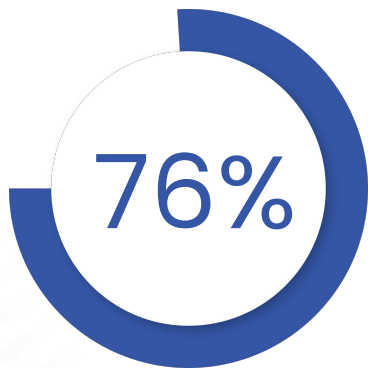
CORA (CodeMate)
